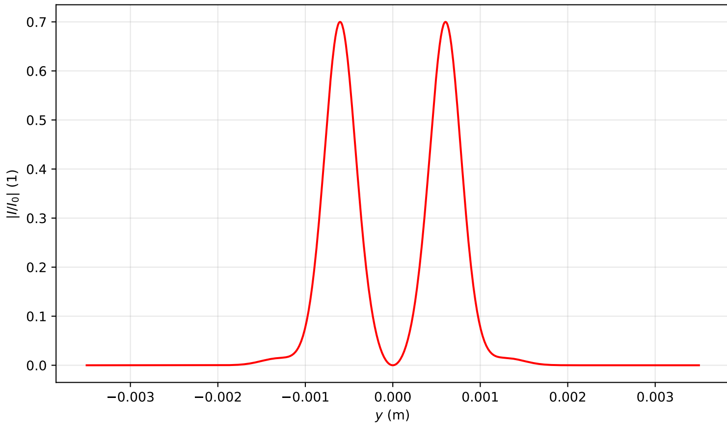
Intensity profile I(x=0, y, z=1.035)/I_0 , P_{in}=4.0P_{cr} , artificial time
